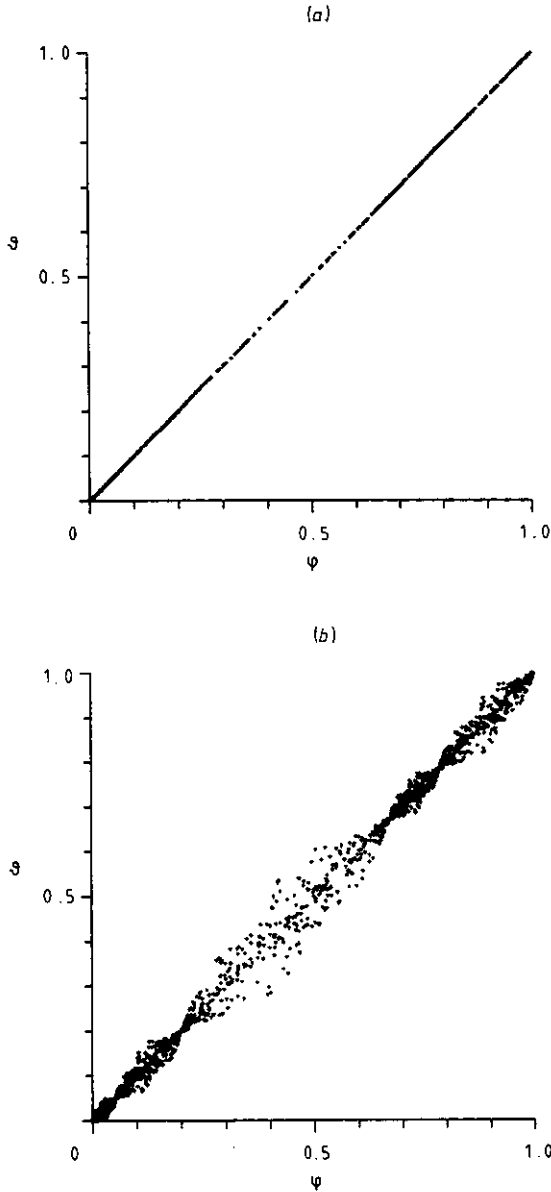
Figure 3. Effect of type-2 coupling on the chaotic motion inside the resonance 3/5: (a) \varepsilon_2 > \varepsilon_{2cr} ; (b) \varepsilon_2 < \varepsilon_{2cr} .
